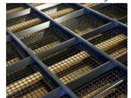
Separator Screen Tray
